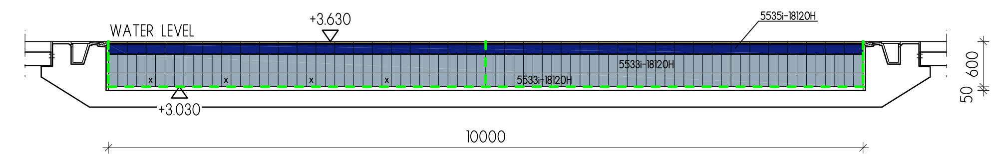
SECTION C - C S: 1:50
