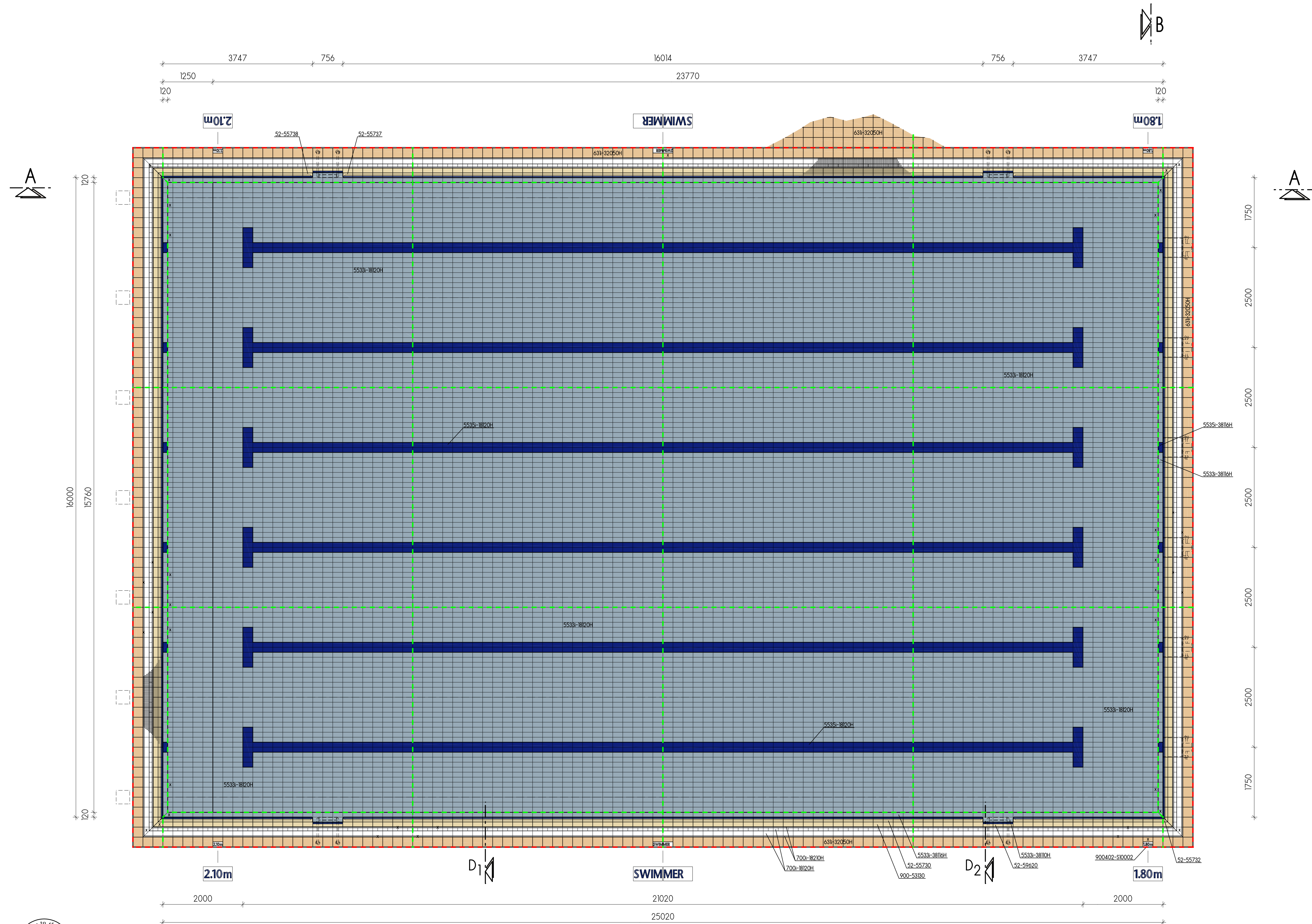
PLAN S: 1:50
