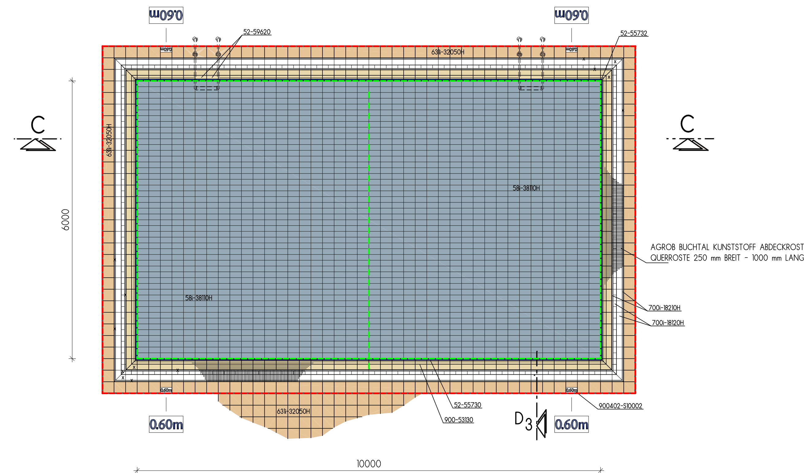
PLAN S: 1:50
